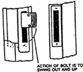
DEAD BOLT LOCK FOR NARROW FRAME DOORS
